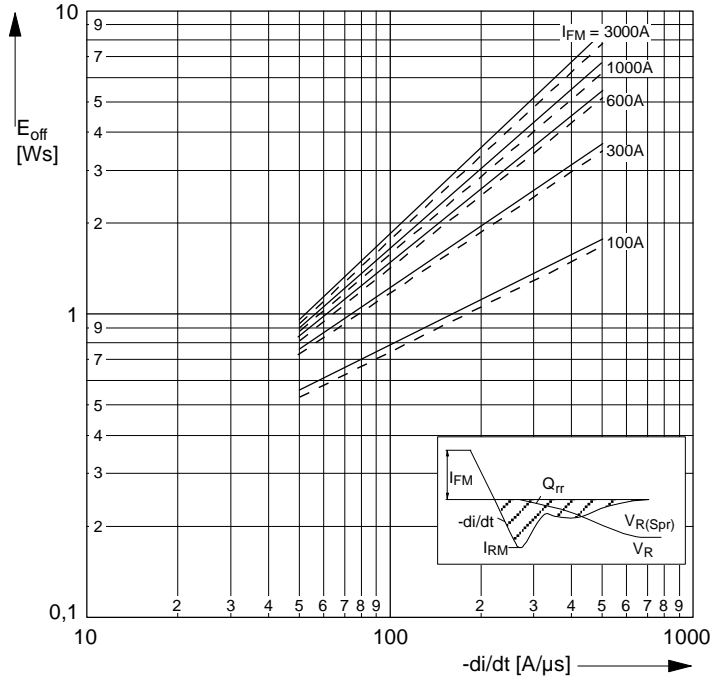
Fig. 11 Turn-off-losses E_{off} = f(di/dt) diodes with V_{Fmax}
