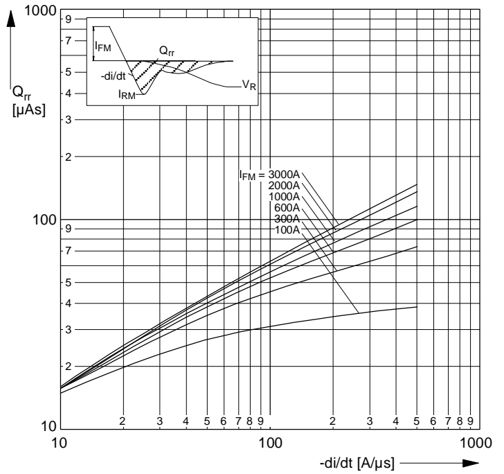
Fig. 9 Reverse recovery charge (lower limit, ca. 2% values)
