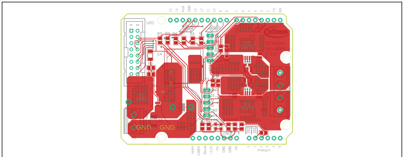
Figure 16 Top layer, top view rev. 2.0
