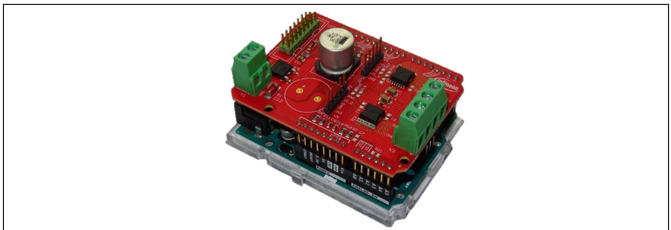
Figure 1 BTN9960/BTN9970/BTN9990 motor control shield stacked on Arduino UNO board
