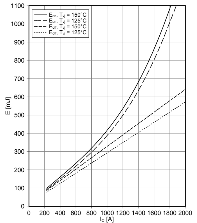
开关损耗 IGBT, 制动-斩波器 (典型) switching losses IGBT, Brake-Chopper (typical) E_{on} = f(I_C) , E_{off} = f(I_C) V_{GE} = \pm 15\text{ V} , R_{Gon} = 1.2\ \Omega , R_{Goff} = 1.8\ \Omega , V_{CE} = 900\text{ V}
