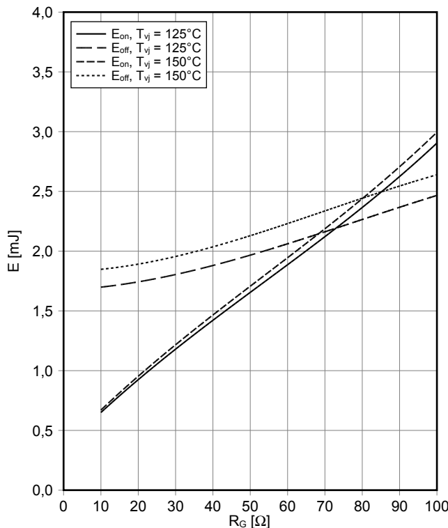
开关损耗 IGBT, 斩波器 (典型) switching losses IGBT-Chopper (typical)
