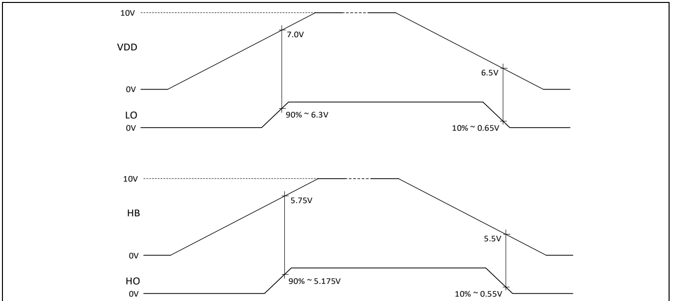
Figure 5 UVLO behavior
