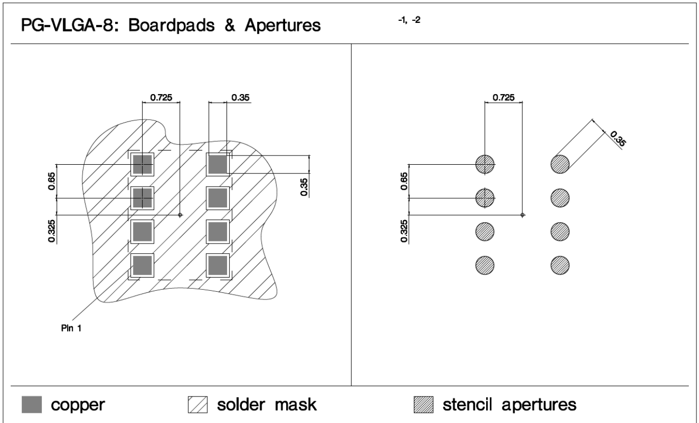
Figure 18 DPS368 footprint and stencil recommendation
