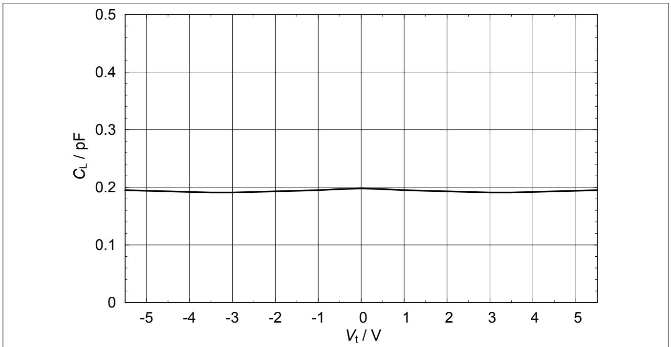
Figure 4 Line capacitance: C_L = f(V_t) , f = 1 MHz
