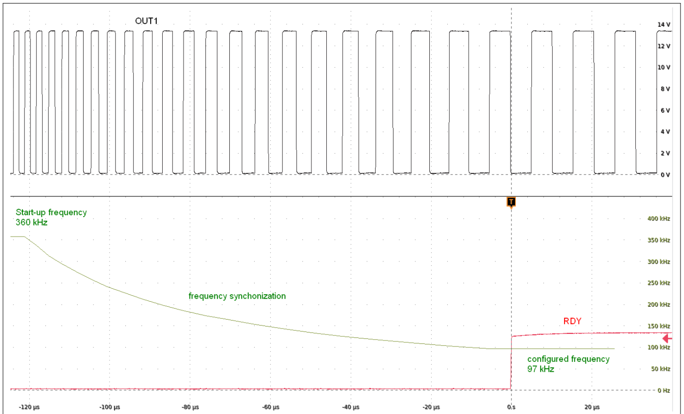
Figure 14 OUT1 switching waveform
