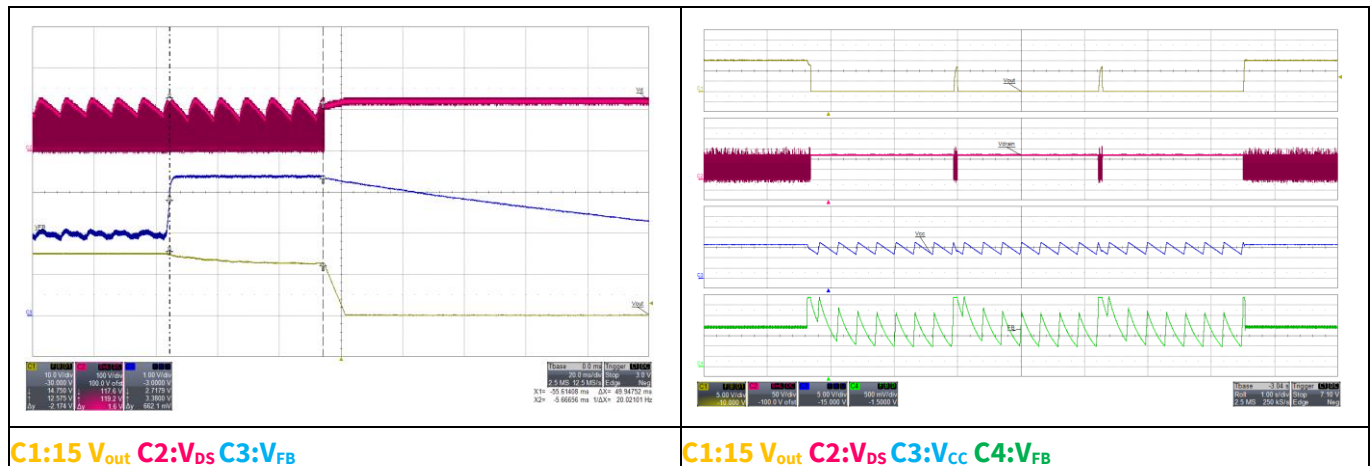
Figure 16 Overload protection
