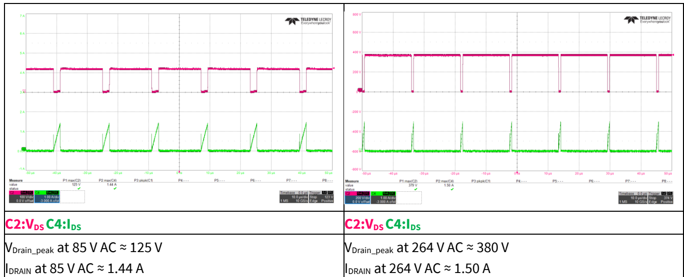
Figure 13 Drain and CS voltage at maximum load
