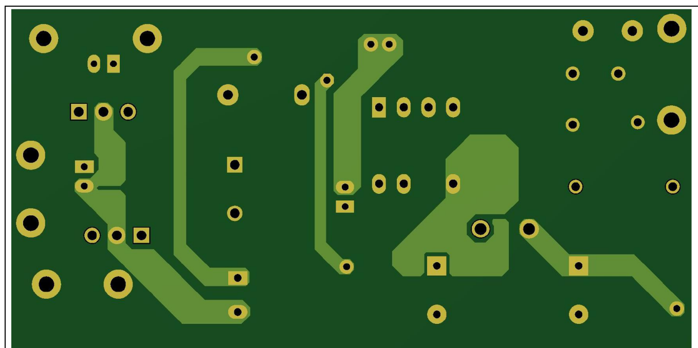
Figure 4 Bottom-side copper
