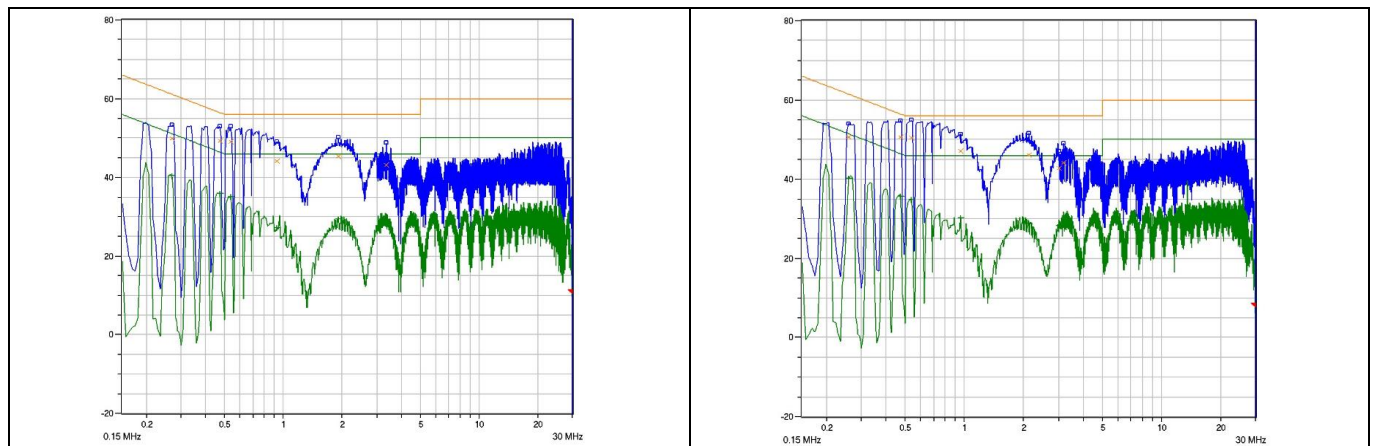
Figure 9 Conducted emissions at 230 V AC with full load
