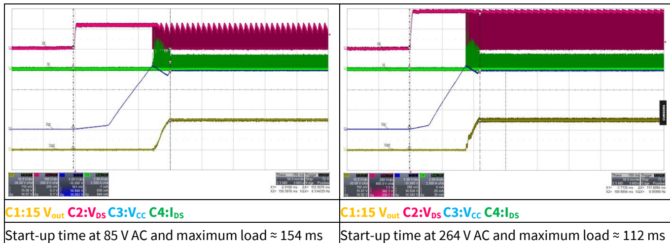
Figure 11 Start-up
