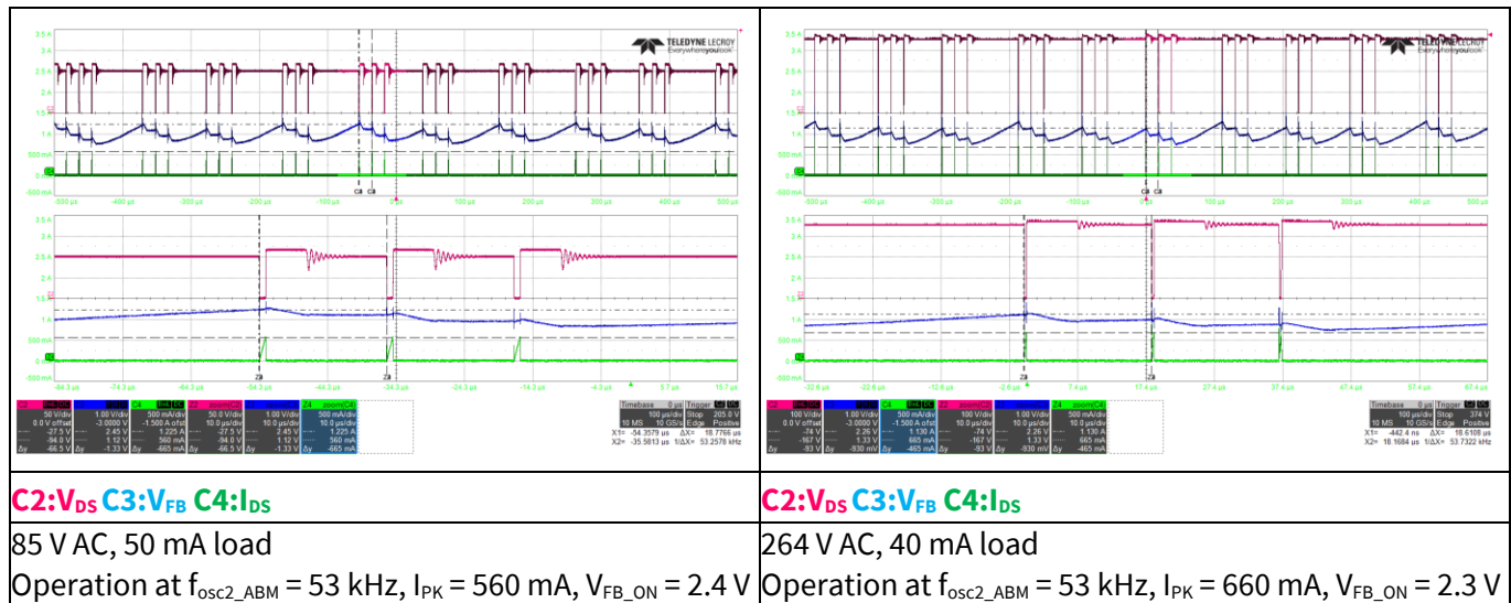
Figure 15 ABM operation
