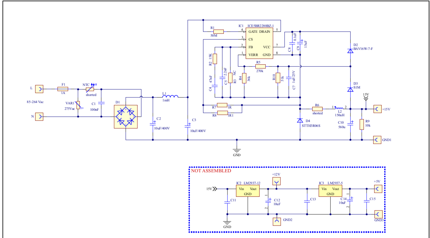
Figure 2 EVAL_5BR2280BZ-1_700mA1
