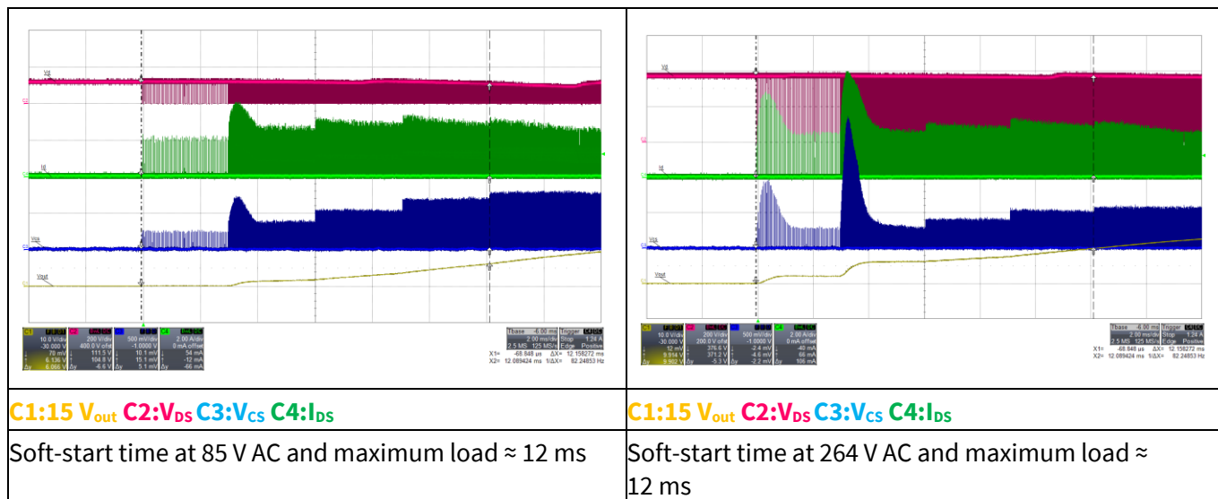
Figure 12 Soft-start
