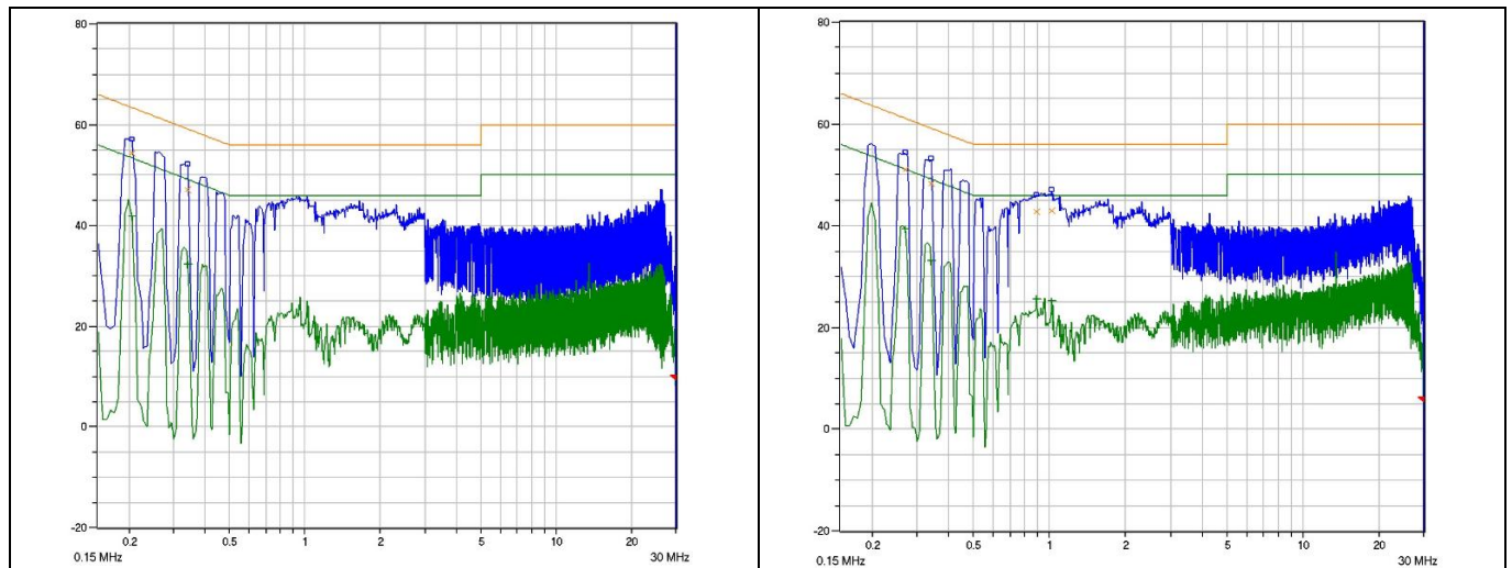
Figure 8 Conducted emissions at 115 V AC with full load
