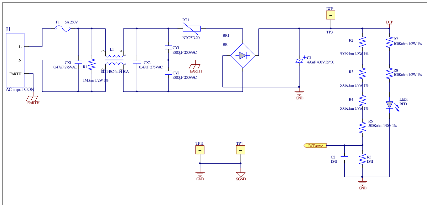
Figure 22 AC Linear Section Schematics for EVAL-M1-CTE610N3
