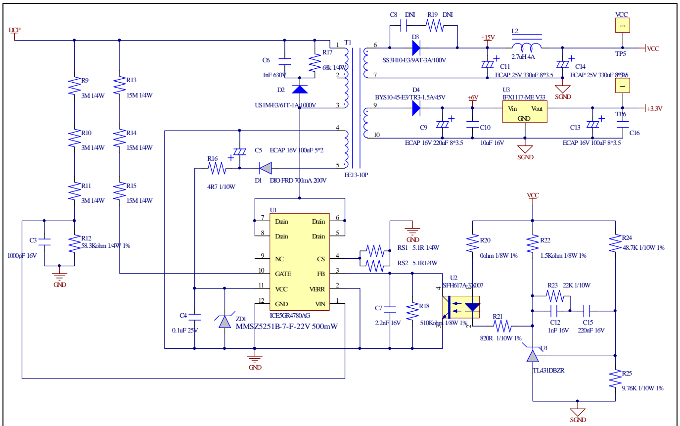
Figure 24 Auxiliary Power Supply Section Schematics for EVAL-M1-CTE610N3
