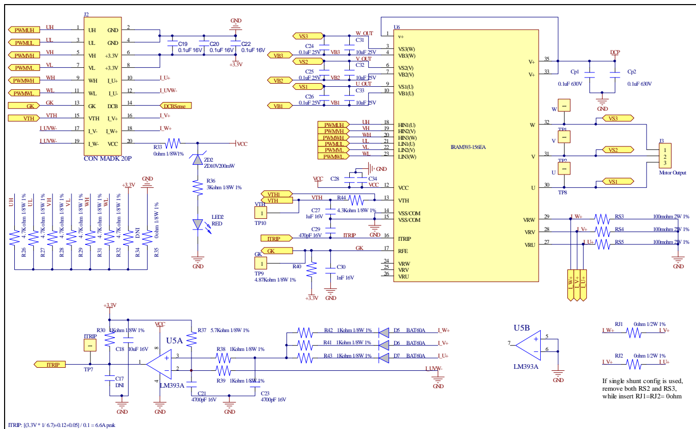
Figure 23 Inverter Section Schematics for EVAL-M1-CTE610N3
