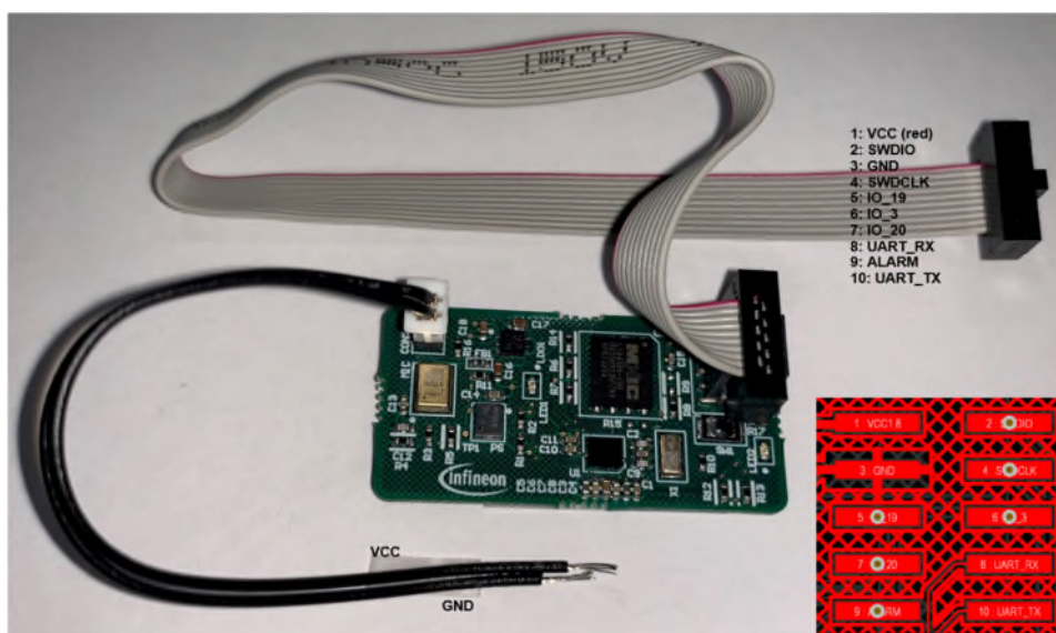
Figure 2 MicroIAS form-factor board connections
