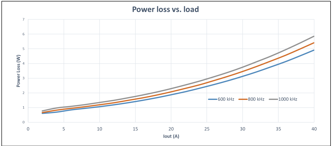
Figure 22 Power loss vs. load current without airflow in FCCM with external V CC (12 V P VIN , 1.2 V V OUT , no airflow, 150 nH, 600 kHz/800 kHz/1000 kHz, T a = 25°C)
