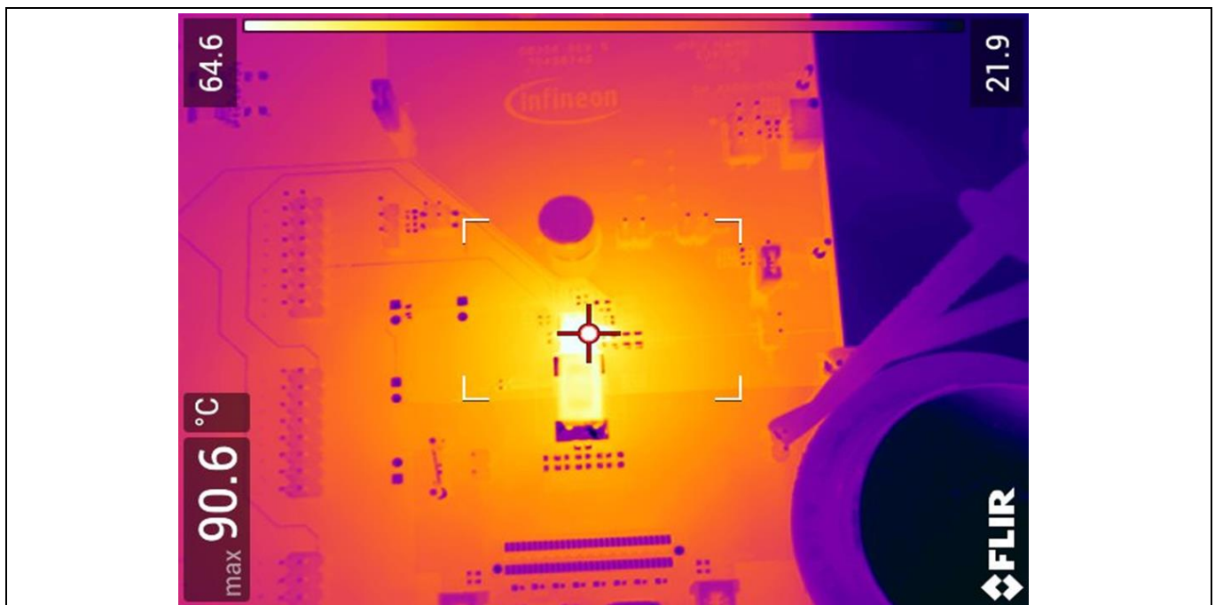
Figure 32 Thermal image of the board at 3.3 V 35 A load TDA38740 = 90.6°C, L = 61.3°C, T a = 22.3°C, natural convection, f sw = 1000 kHz
