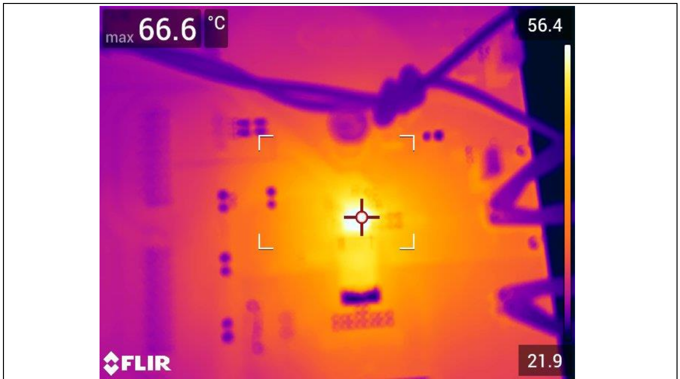
Figure 23 Thermal image of the board at 1.2 V 40 A load TDA38740 = 66.6°C, L = 47.3°C, T a = 21.9°C, natural convection, f sw = 1000 kHz
