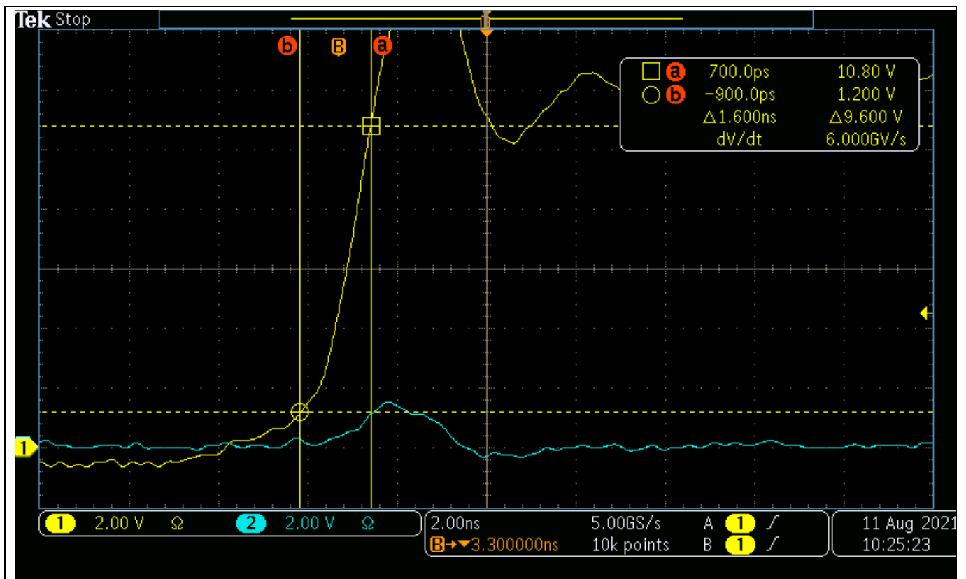
Figure 28 SW and GL, 30 A load, f sw = 800 kHz
