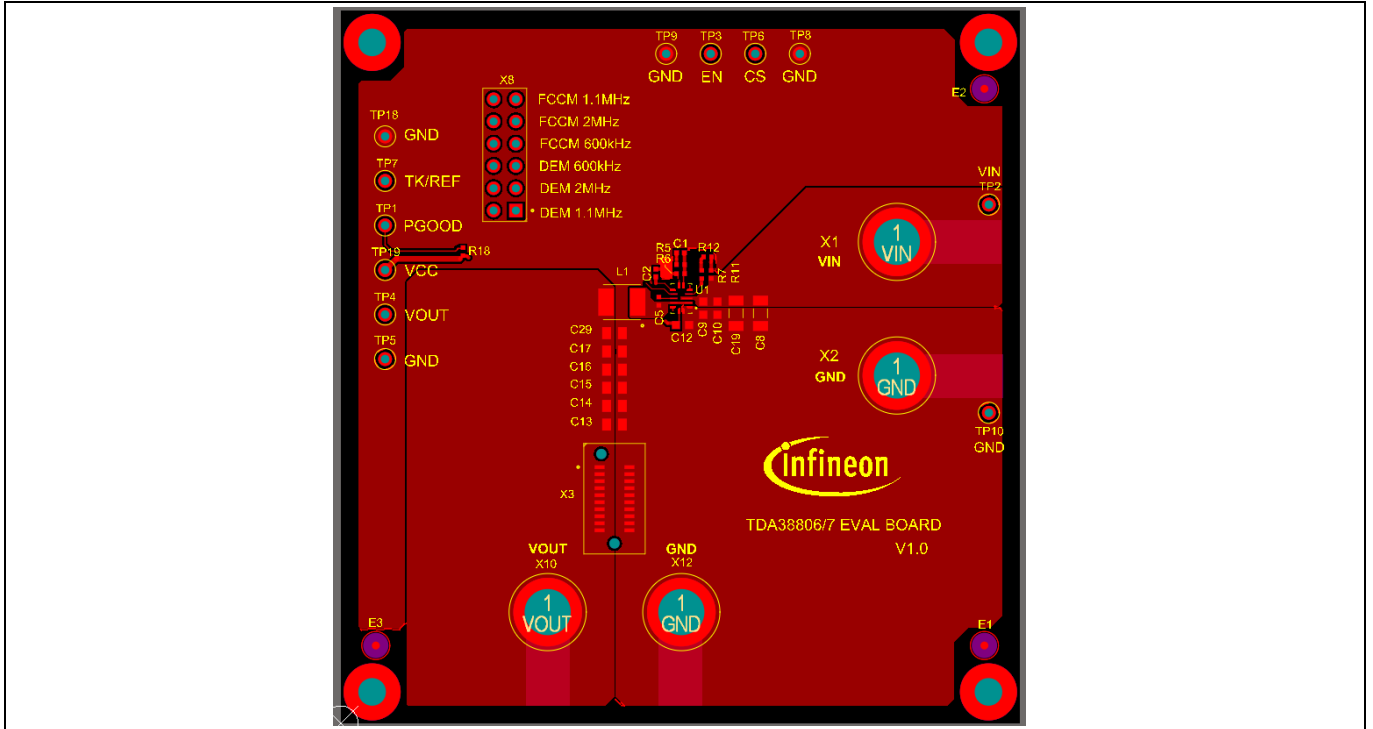
Figure 1 Top Layer
