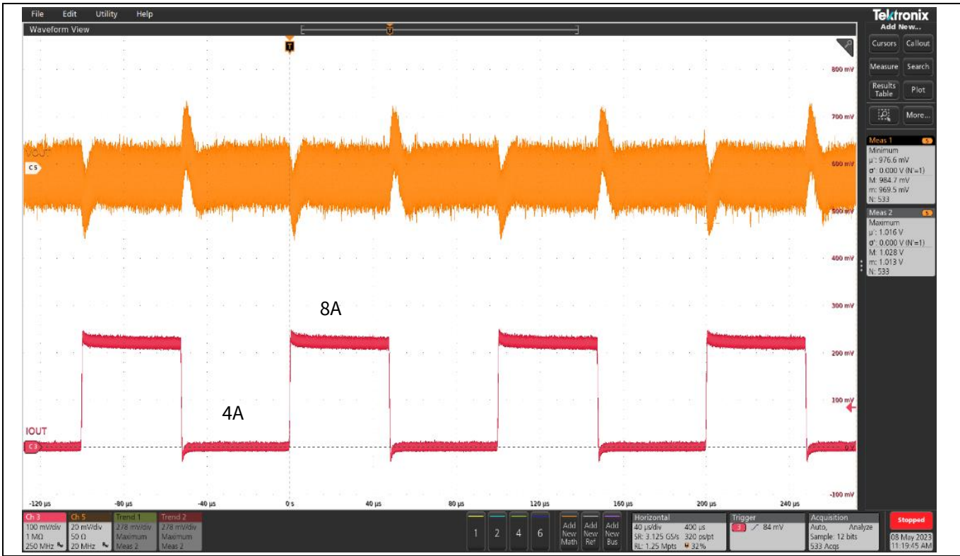
Figure 17 Transient response at 4 A step load current at 10 A/ \mu s slew rate: I OUT = 4 A – 8 A, (Ch5: V OUT , Ch3: I OUT ), pk-pk: 39.4mV, F SW = 800 kHz
