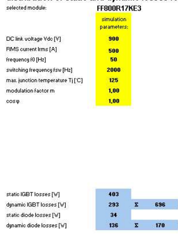
IGBT Power Simulation for Infineon IGBT modules V6.1a September 2006 module selection for 3-phase inverter applications
