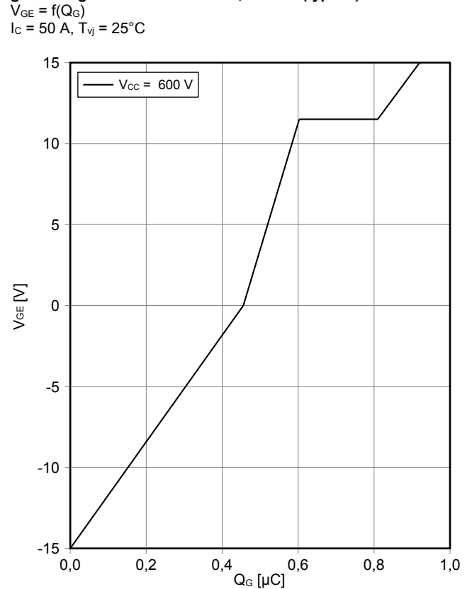
Gateladungs Charakteristik IGBT, Wechselrichter (typisch) gate charge characteristic IGBT, Inverter (typical) V_{GE} = f(Q_G) I_C = 50\text{ A} , T_{vj} = 25^\circ\text{C}
