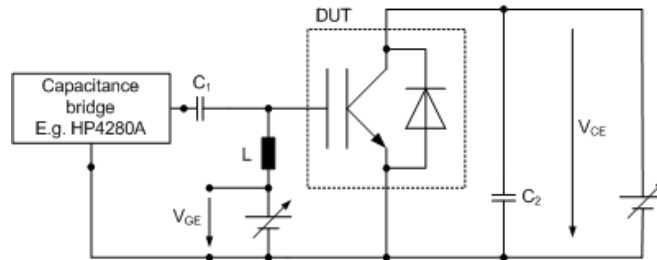
Figure 13: Basic circuit diagram for measuring the input capacitance C_{ies}
