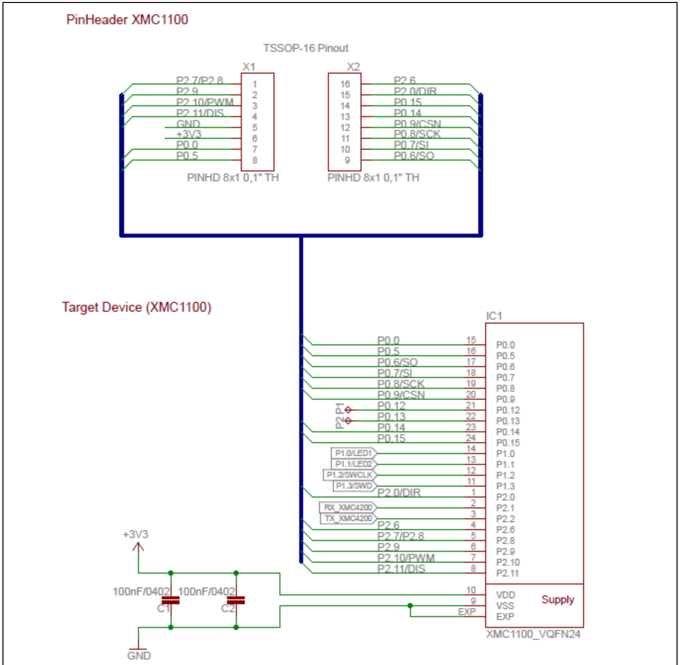
Figure 16 XMC1100 and Pin Header
