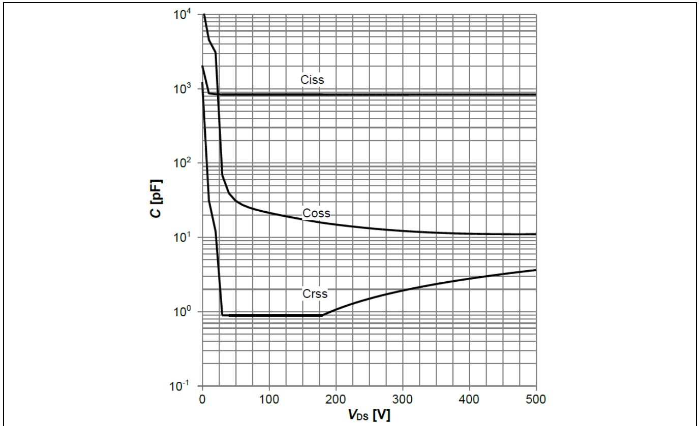
Figure 26 Typical CoolMOS™ capacitances of ICE5QR0680BG ( C=f(V_{DS}); V_{GS}=0\text{ V}; f=250\text{ kHz} )
