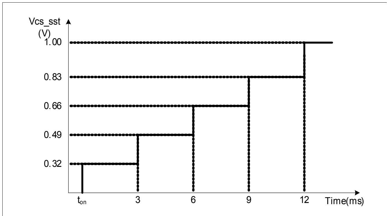
Figure 5 Maximum current sense voltage during softstart
