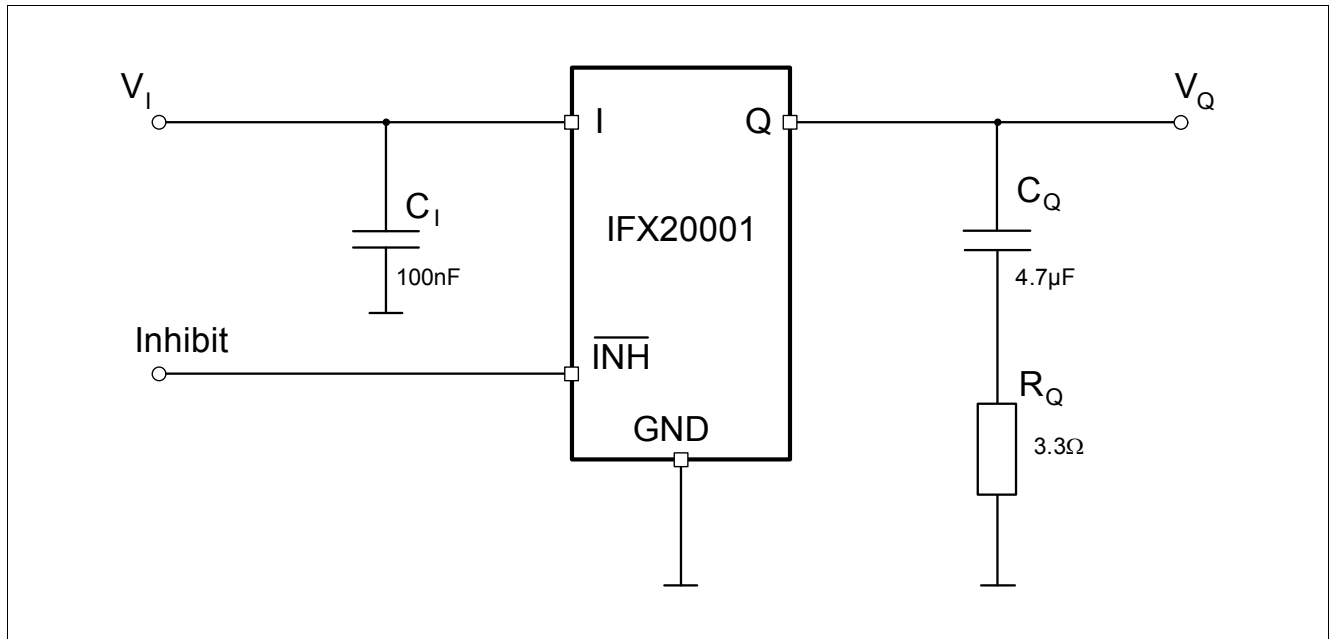
Figure 3 Application Diagram
