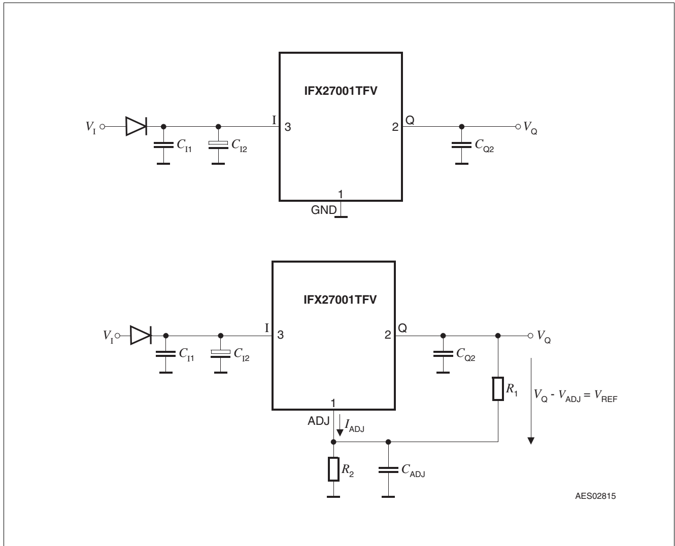
Figure 5 Application Diagram
