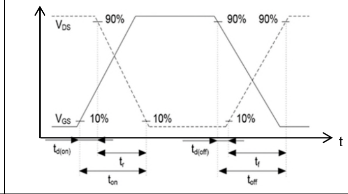
Figure 24 Switching times waveform
