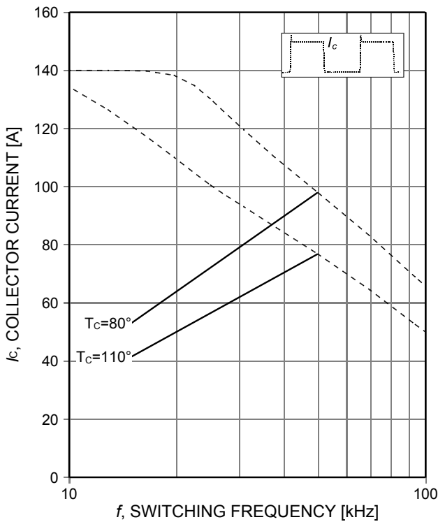
Figure 1. Collector current as a function of switching frequency ( T_{vj} \leq 175^\circ\text{C} , D=0.5 , V_{CE}=400\text{V} , V_{GE}=15/0\text{V} , r_G=3.5\Omega , R_{th(j-c)}=0.21\text{K/W} )
