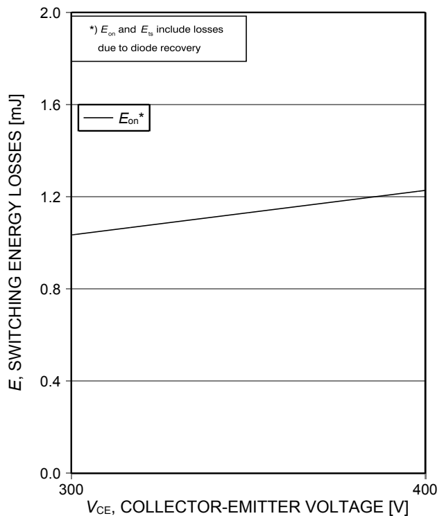
Figure 16. Typical switching energy losses as a function of collector emitter voltage (inductive load, T_j=175^\circ\text{C} , V_{GE}=0/15\text{V} , I_C=40\text{A} , R_{G(\text{on})}=5.6\Omega , R_{G(\text{off})}=5.6\Omega , dynamic test circuit in Figure E)
