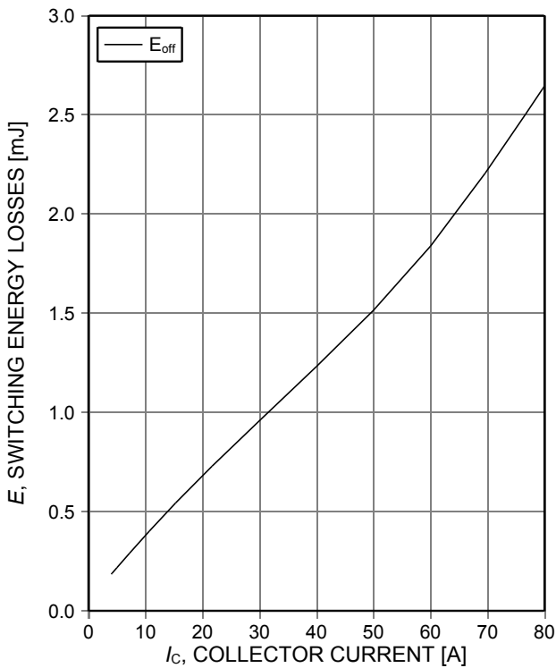
Figure 13. Typical switching energy losses as a function of collector current (inductive load, T_j=175^\circ\text{C} , V_{CE}=400\text{V} , V_{GE}=0/15\text{V} , R_{G(\text{on})}=5.6\Omega , R_{G(\text{off})}=5.6\Omega , dynamic test circuit in Figure E)
