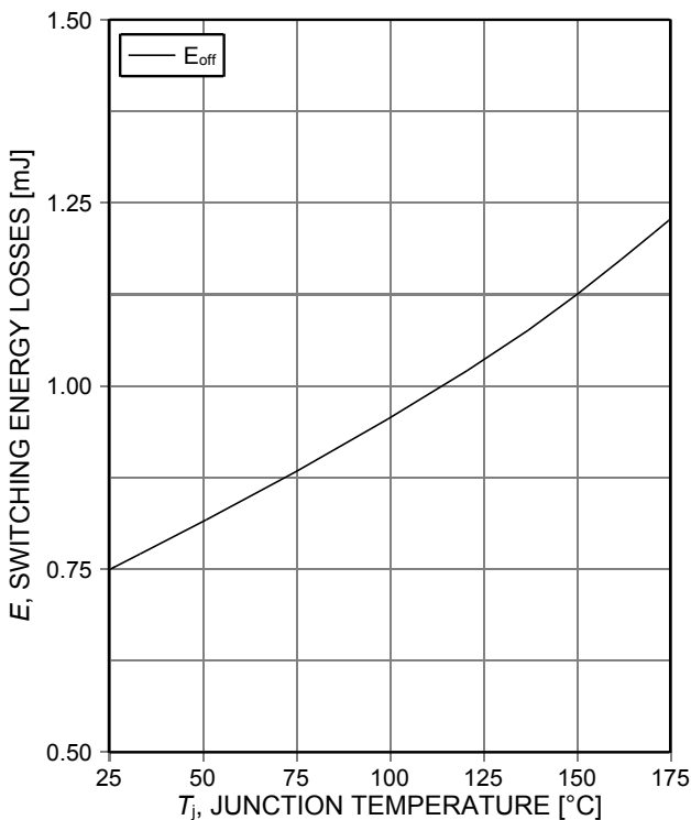
Figure 15. Typical switching energy losses as a function of junction temperature (inductive load, V_{CE}=400\text{V} , V_{GE}=0/15\text{V} , I_C=40\text{A} , R_{G(\text{on})}=5.6\Omega , R_{G(\text{off})}=5.6\Omega , dynamic test circuit in Figure E)
