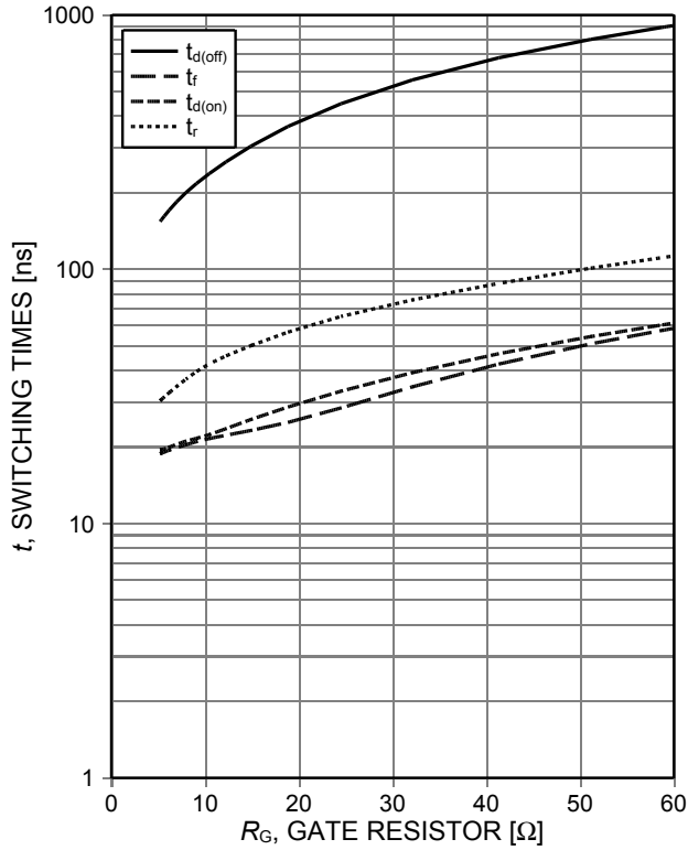
Figure 9. Typical switching times as a function of gate resistor (ind. load, T_j=175^{\circ}\text{C} , V_{\text{CE}}=400\text{V} , V_{\text{GE}}=0/15\text{V} , I_{\text{C}}=40\text{A} , test circuit in Fig. E)
