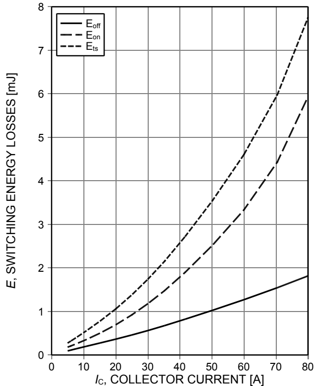
Figure 12. Typical switching energy losses as a function of collector current (ind. load, T_j=175^{\circ}\text{C} , V_{\text{CE}}=400\text{V} , V_{\text{GE}}=0/15\text{V} , R_{\text{G}}=8\Omega , test circuit in Fig. E)
