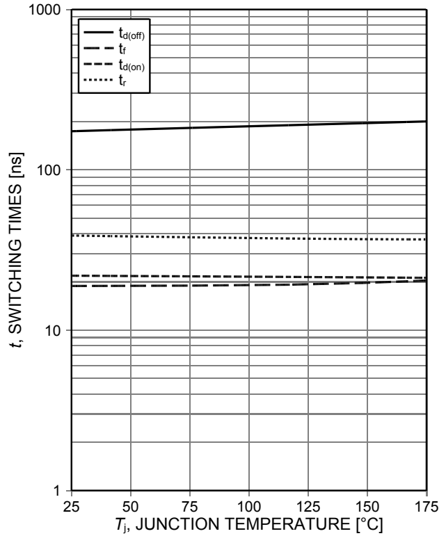
Figure 10. Typical switching times as a function of junction temperature (ind. load, V_{\text{CE}}=400\text{V} , V_{\text{GE}}=0/15\text{V} , I_{\text{C}}=40\text{A} , r_{\text{G}}=8\Omega , test circuit in Fig. E)
