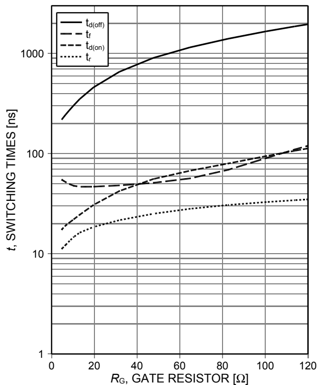
Figure 8. Typical switching times as a function of gate resistor (inductive load, T_{vj}=175^{\circ}C , V_{CE}=400V , V_{GE}=15/0V , I_C=30A , Dynamic test circuit in Figure E)
