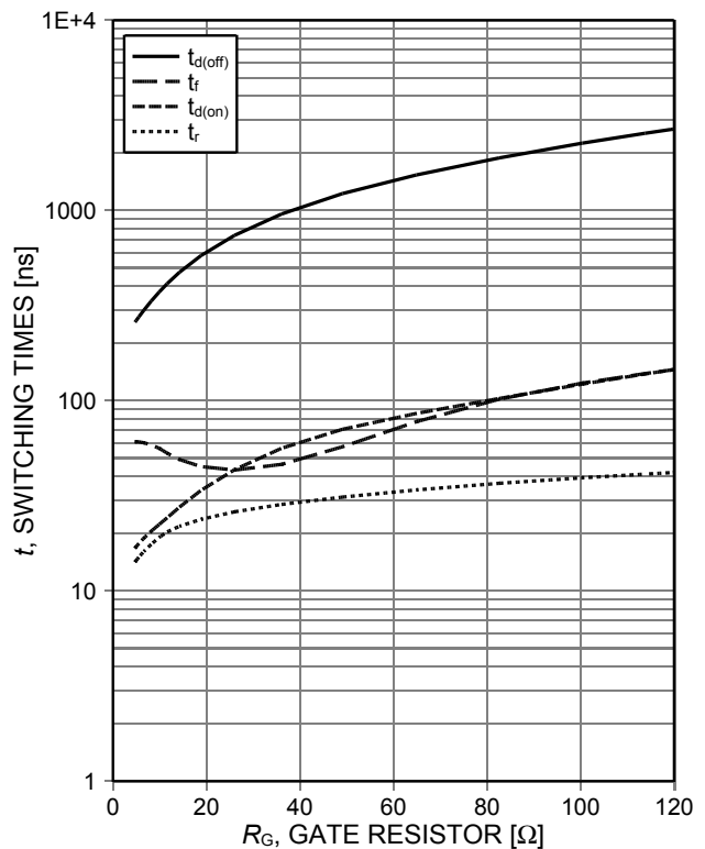
Figure 8. Typical switching times as a function of gate resistor (inductive load, T_{vj}=175^{\circ}C , V_{CE}=400V , V_{GE}=15/0V , I_C=40A , Dynamic test circuit in Figure E)
