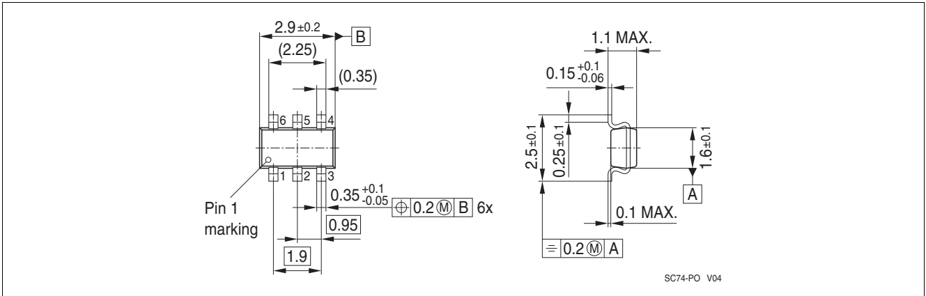
Figure 7 Package Outline SC74
