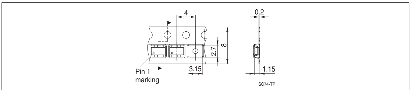
Figure 9 Tape Loading
