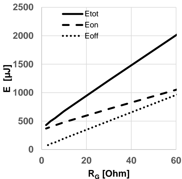
Figure 17 Typical switching energy losses as a function of gate resistance ( E = f(R_{G,ext}) , V_{DD} = 800V , V_{GS} = 0V/18V , I_D = 16A , T_{vj} = 175^\circ C , ind. load, test circuit in Fig. E, diode: body diode at V_{GS} = 0V )
