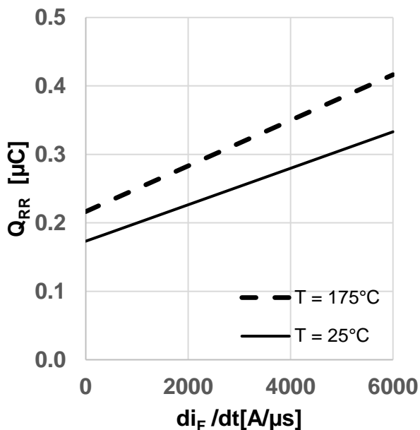
Figure 19 Typical reverse recovery charge as a function of diode current slope ( Q_{rr} = f(di_i/dt) , V_{DD} = 800V , V_{GS} = 0V/18V , I_D = 16A , ind. load, test circuit in Fig.E, body diode at V_{GS} = 0V )
