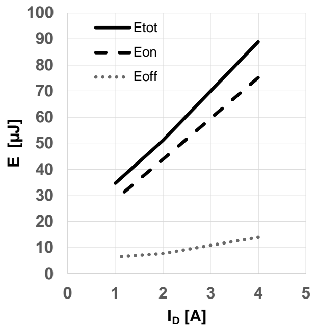
Figure 16 Typical switching energy losses as a function of drain-source current (E = f(I_{DS}), V_{DD} = 800\text{V}, V_{GS} = 0\text{V}/18\text{V}, R_{G,ext} = 2\Omega, T_{vj} = 175^{\circ}\text{C}, \text{ind. load, test circuit in Fig. E, diode: body diode at } V_{GS} = 0\text{V})
