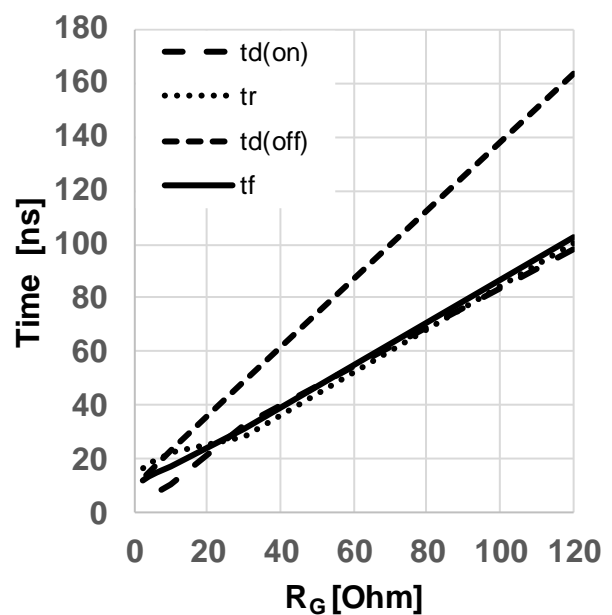
Figure 18 Typical switching times as a function of gate resistor ( t = f(R_{G,ext}), V_{DD} = 800V, V_{GS} = 0V/18V, I_D = 13A, T_{vj} = 175^\circ C, ind. load, test circuit in Fig. E, diode: body diode at V_{GS} = 0V )
