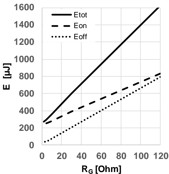
Figure 17 Typical switching energy losses as a function of gate resistance ( E = f(R_{G,ext}), V_{DD} = 800V, V_{GS} = 0V/18V, I_D = 13A, T_{vj} = 175^\circ C, ind. load, test circuit in Fig. E, diode: body diode at V_{GS} = 0V )
