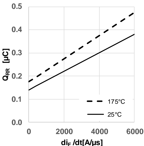
Figure 19 Typical reverse recovery charge as a function of diode current slope ( Q_{rr} = f(di_i/dt), V_{DD} = 800V, V_{GS} = 0V/18V, I_D = 13A, ind. load, test circuit in Fig.E, body diode at V_{GS} = 0V )
