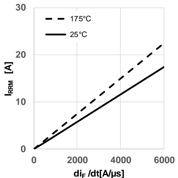
Figure 20 Typical reverse recovery current as a function of diode current slope ( I_{rrm} = f(di_i/dt), V_{DD} = 800V, V_{GS} = 0V/18V, I_D = 13A, ind. load, test circuit in Fig.E, body diode at V_{GS} = 0V )
