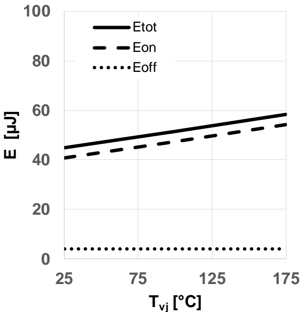
Figure 15 Typical switching energy losses as a function of junction temperature ( E = f(T_{vj}) , V_{DD} = 800V , V_{GS} = 0V/18V , R_{G,ext} = 2\Omega , I_D = 2A , ind. load, test circuit in Fig. E, diode: body diode at V_{GS} = 0V )
