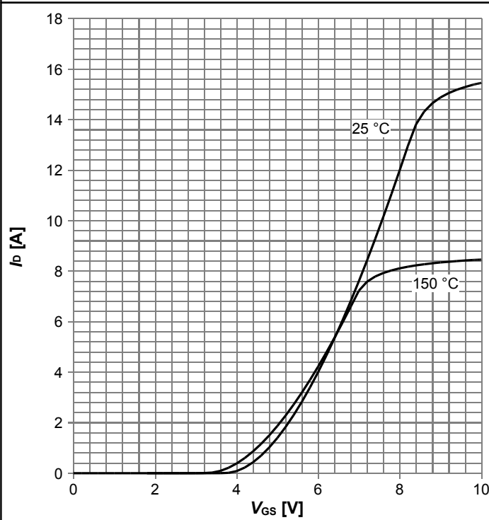
Typ. transfer characteristics
