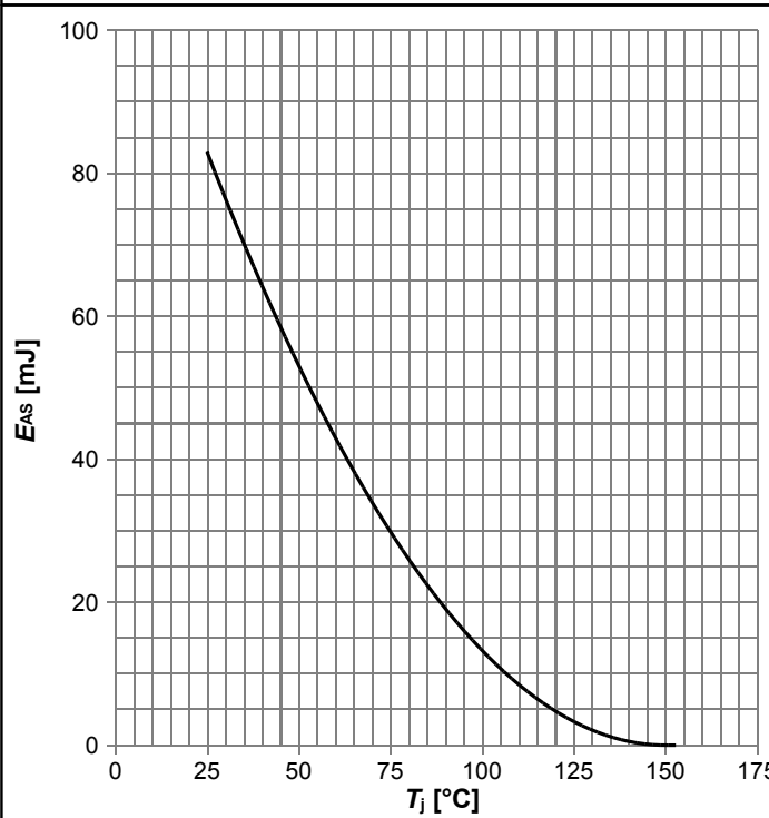
Avalanche energy
