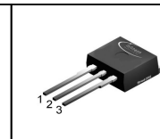
PG-TO262-3-1
