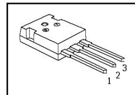
PG-TO247-3
