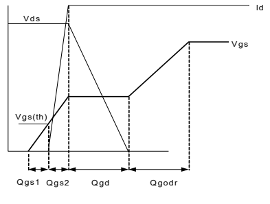
Fig 18b. Gate Charge Waveform
