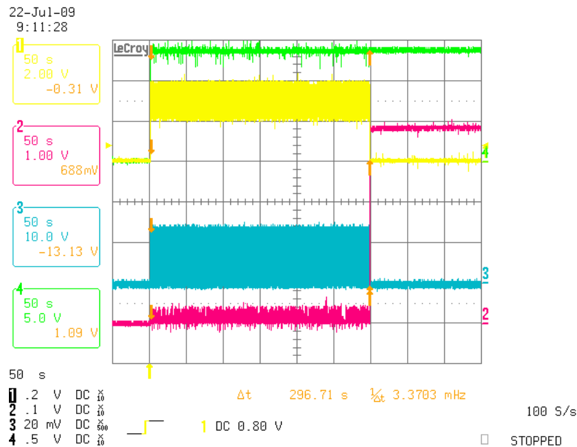
Figure 6.2: Under-voltage fault: CH1 is CLK pin voltage, CH2 is VSENSE voltage, CH3 is LO voltage and CH4 is VCC voltage
