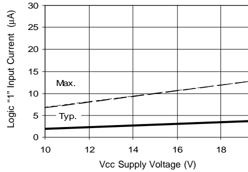
Figure 16B. Logic "1" Input Current vs. Voltage
