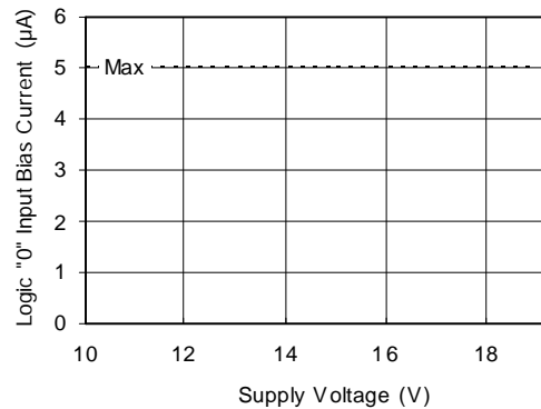
Figure 17B. Logic "0" Input Current vs. Voltage
