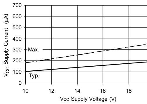
Figure 15B. V CC Supply Current vs. Voltage
