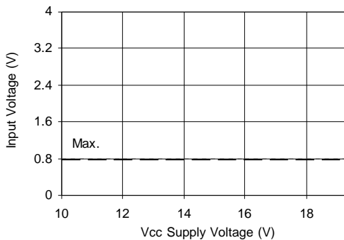
Figure 10B. Logic "0" (HIN) & Logic "1" (LIN) Input Voltage vs. Voltage
