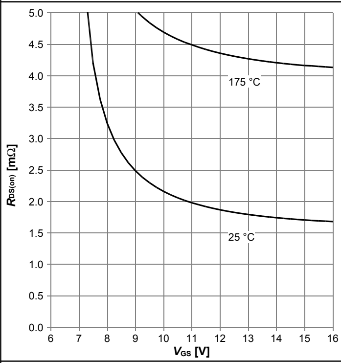
Diagram 9: Typ. drain-source on resistance
