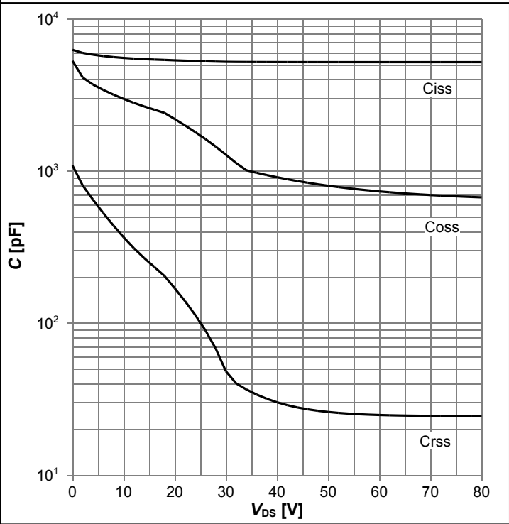
Diagram 12: Typ. capacitances
