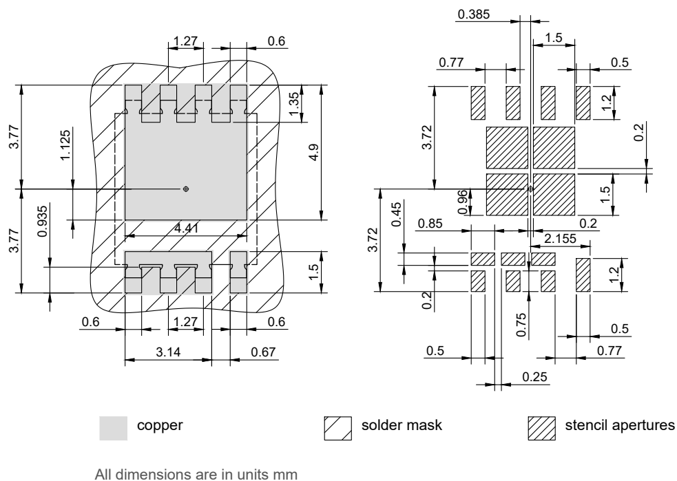
Figure 2 Outline PG-TDSON-8, dimensions in mm
