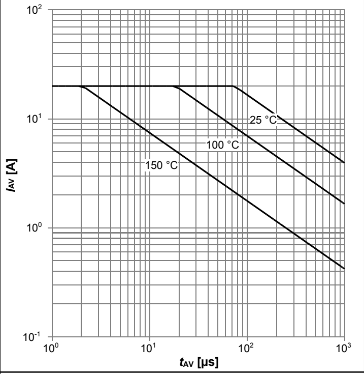
Diagram 14: Avalanche characteristics
