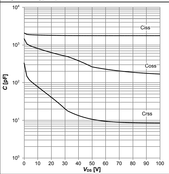
Diagram 12: Typ. capacitances
