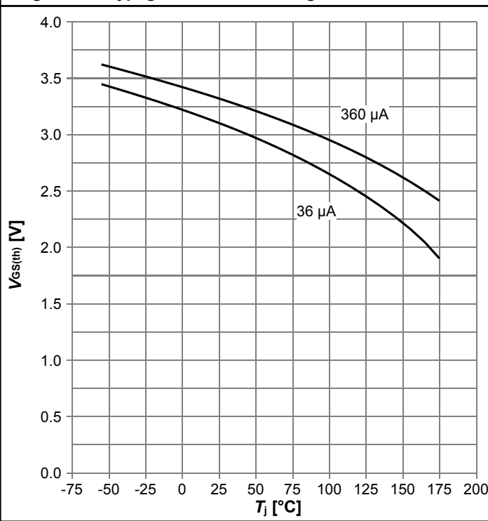
Diagram 11: Typ. gate threshold voltage
