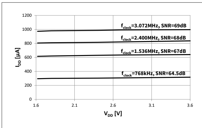
Figure 6 Typical I_{DD} vs V_{DD}
