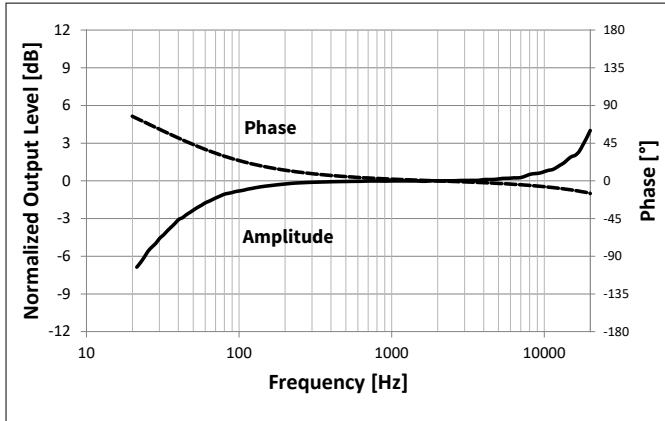
Figure 2 Typical amplitude and phase response
