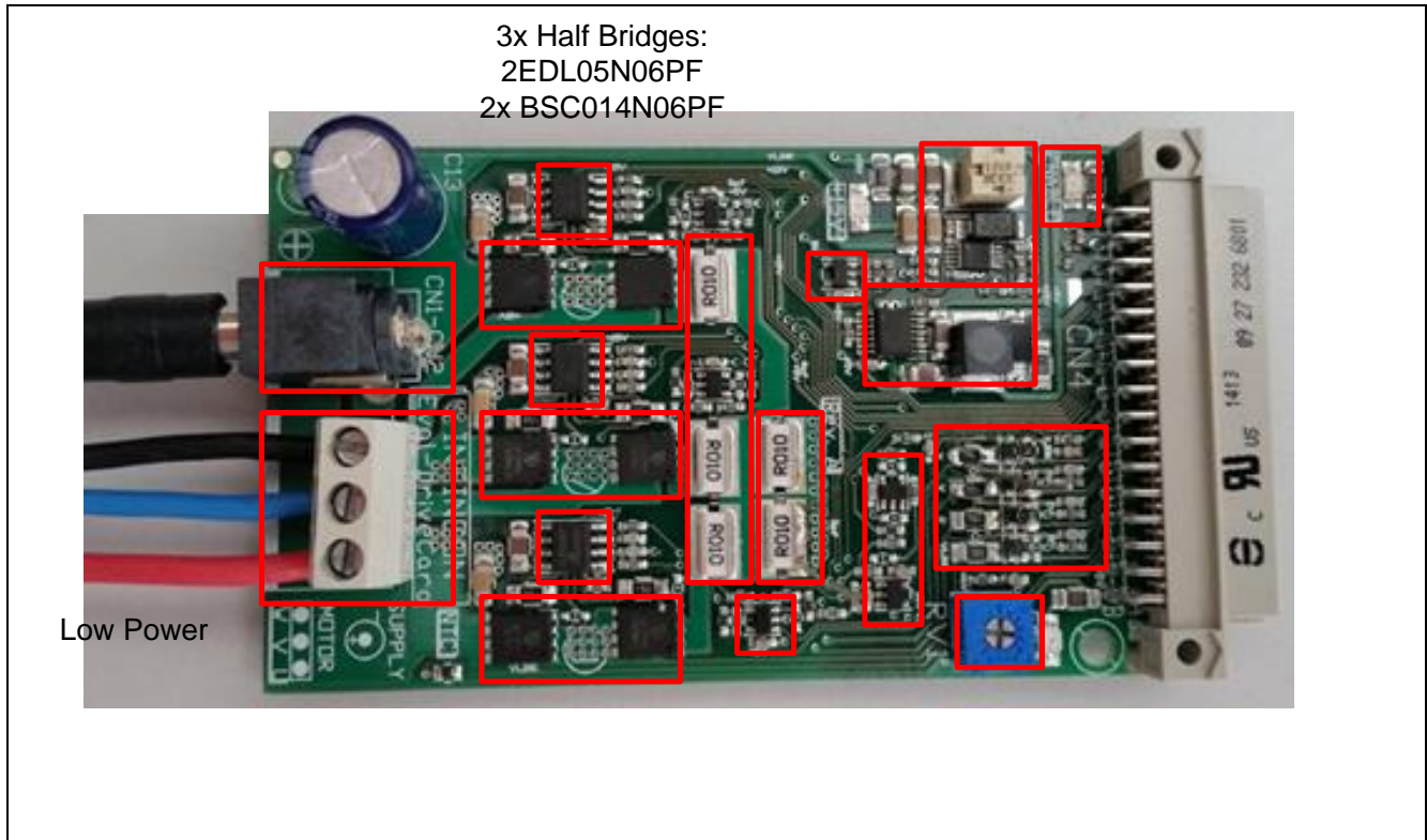
5 Figure 2 Hardware TOP overview
