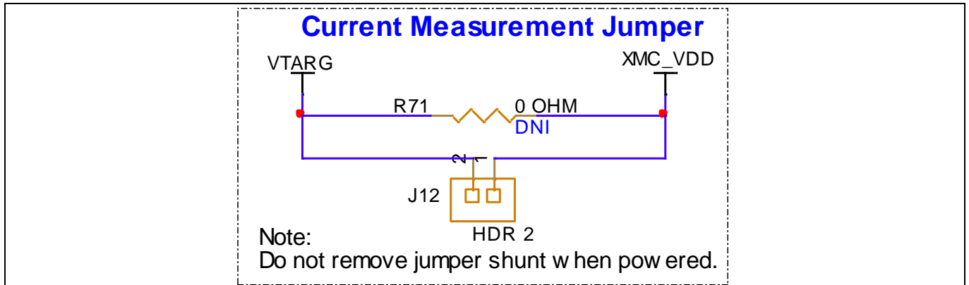
Figure 25 Current measurement headers
