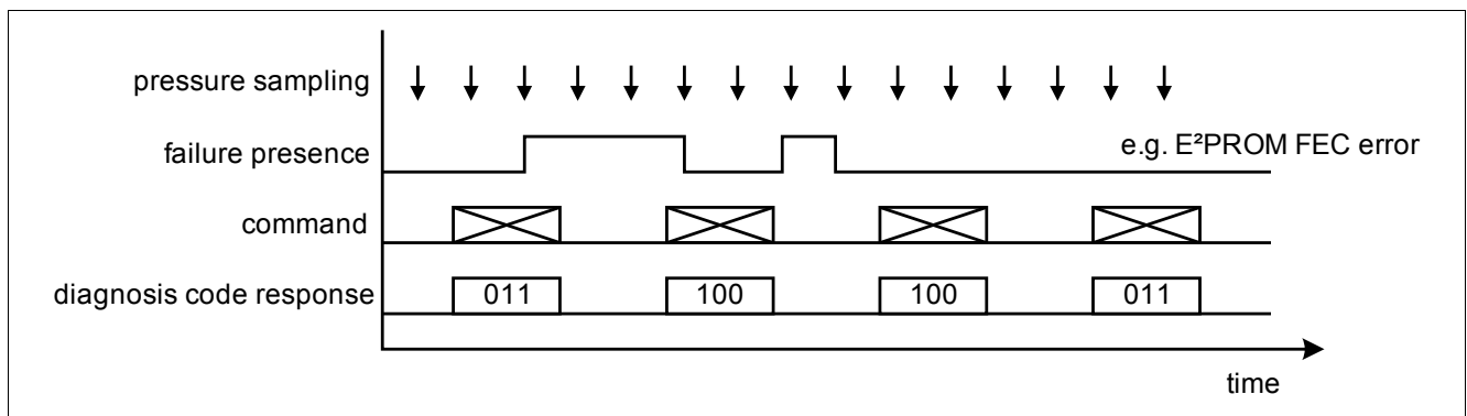
Figure 22 Example for reset strategy Reset-bit C12 = '0'
