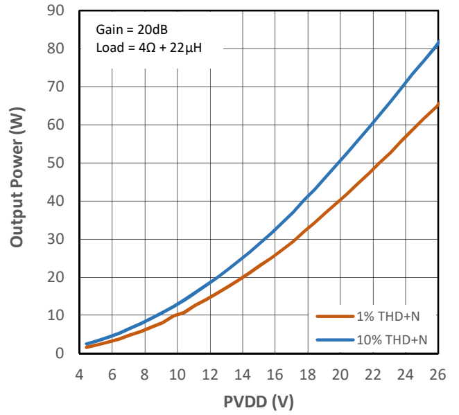
Figure 10-22 Output Power vs PVDD Voltage for PMP1
