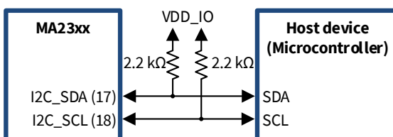
Figure 11.18: I2C serial control interface block diagram
