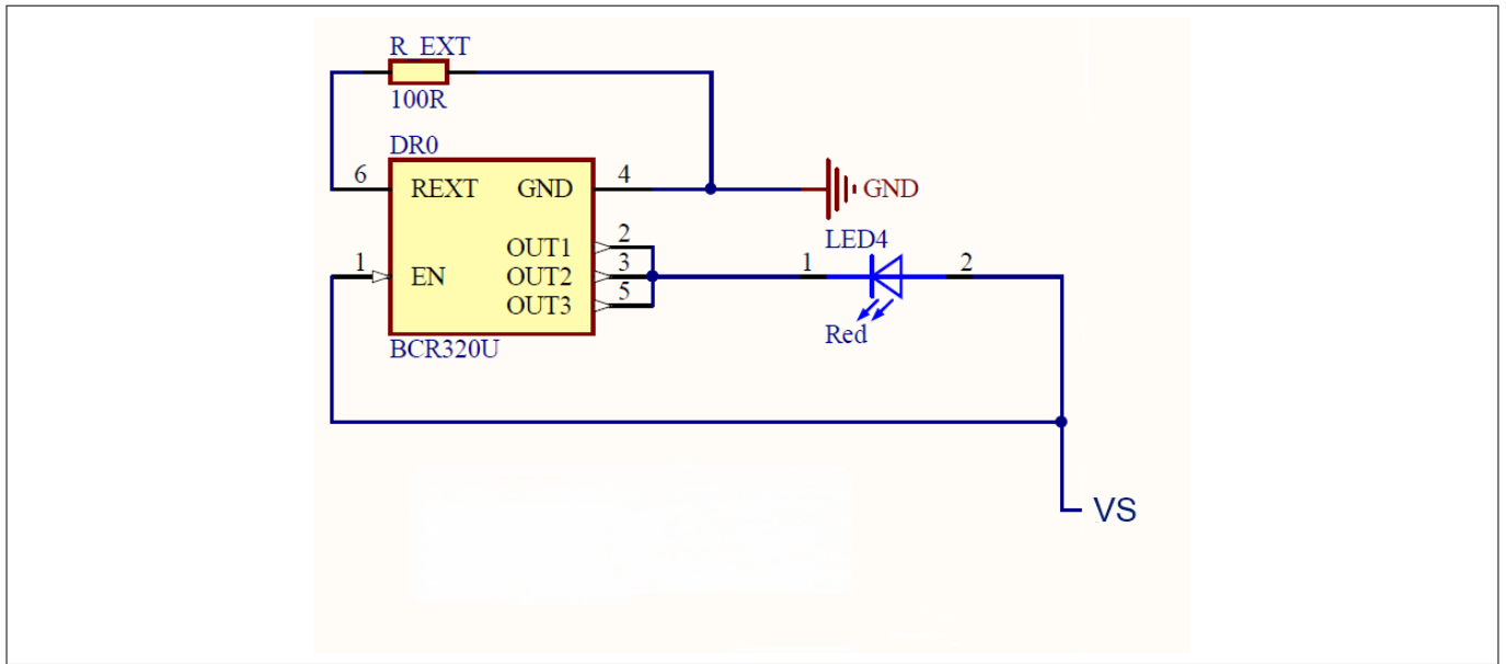
Figure 25 BCR320U circuit
